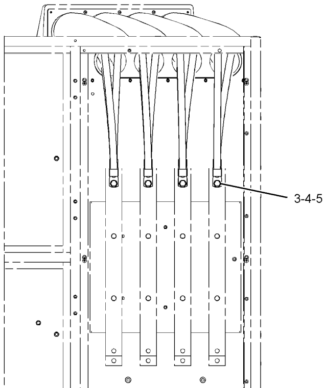
REAR VIEW
