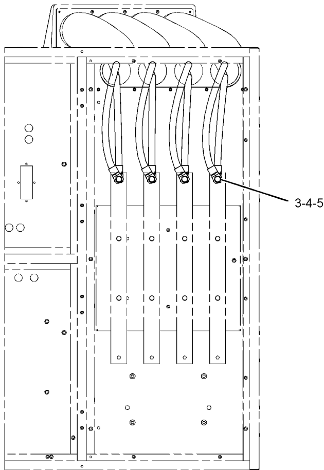
REAR VIEW
